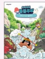
Processes that Shape the Earth
